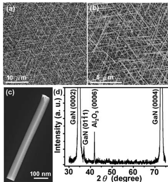
Figure 1. Morphological characterization of GaN NW arrays and crystallographic relationship between GaN NW arrays and GaN/sapphire substrate. (a, b) Low-magnification and high-magnification SEM images of 3-fold symmetrically distributed GaN NW arrays epitaxially grown on GaN/sapphire substrate. (c) Top-view SEM image of a single GaN NW with a triangular cross section. (d) XRD spectrum of GaN NW arrays indicating the epitaxial relationship between GaN NW arrays and GaN/sapphire substrate.
