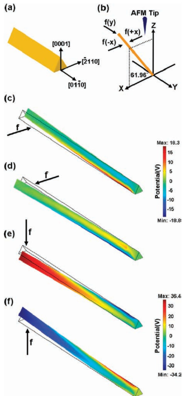
Figure 4. (a) Detailed crystal structure of GaN NW with triangular cross-section utilized for calculation of piezoelectric potential distribution. (b) Coordinate system used to define the direction of lateral force applied from the AFM tip. (c–f) Calculated piezoelectric potential distribution for the GaN NW. The dimension of the NW is the base of NW = 50 nm, length = 10 \mu\text{m} , applied lateral force = 80 nN.
