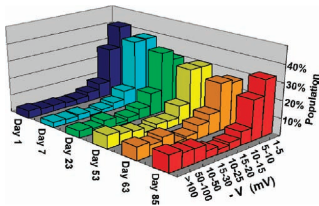
Figure 6. Statistical distribution of the piezoelectric output measured from the same GaN NW arrays sample as a function of time to test the stability and reproducibility.
