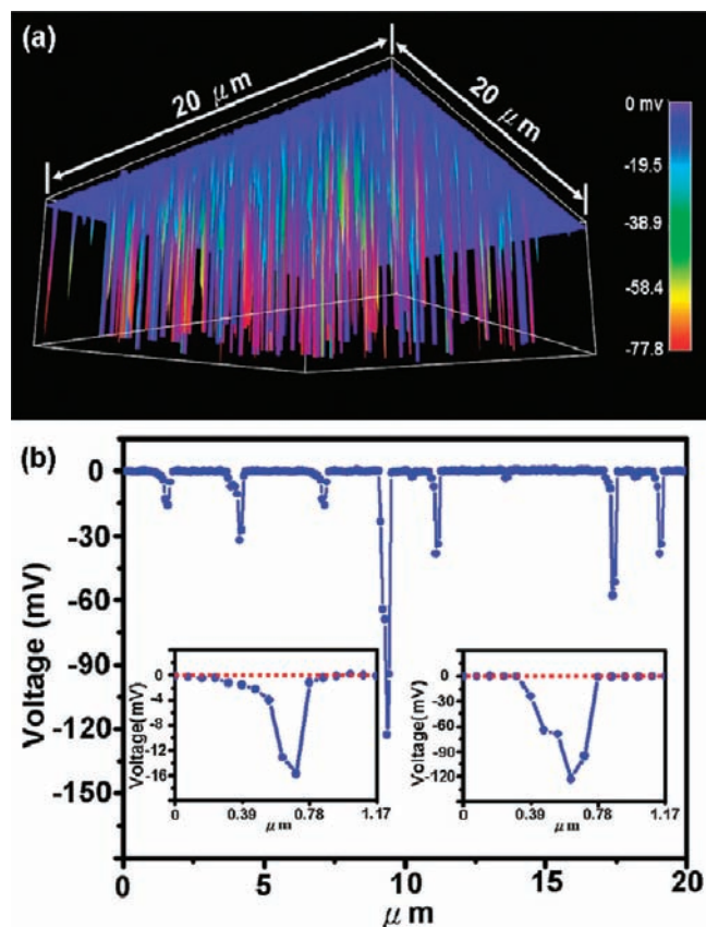
Figure 5. Piezoelectric power generation using the GaN NW arrays. (a) Three-dimensional plot of the output voltage recorded at an external load when the AFM tip scanned and deflected the NW arrays. (b) A typical line scan profile of the output voltage. Insets show the detailed line profile of individual output peaks with high and low output voltages.
