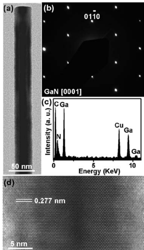
Figure 2. Crystal structures and compositions of GaN NW. (a) Low-magnification TEM image of GaN NW. (b) Corresponding SAED of GaN NW with [0001] zone axis. The growth direction of GaN NW is along the [0110]. (c) Corresponding EDS spectra acquired from GaN NW. (d) Atomic resolution TEM image of GaN NW taken along the [0001] zone axis.
