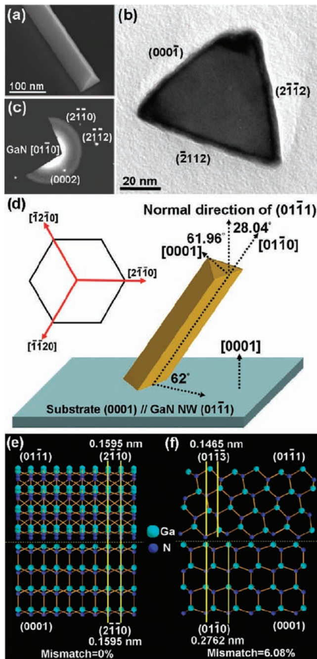
Figure 3. Morphological characterization and crystal structures of GaN NW with a triangular cross section. (a) 30° tilt view SEM image of GaN NW with a triangular cross section. (b) Cross-sectional TEM image of GaN NW enclosed by (0001), (2112), and (2̄112) planes. (c) Corresponding SAED of GaN NW recorded along the [0110] zone axis. (d) Schematic diagram showing crystallographic relationship between GaN NW and GaN/sapphire substrate. The inset is the model for forming the 3-fold symmetric distribution of NWs on the substrate. (e, f) Atomic model exhibiting the epitaxial relationship between GaN NW and GaN/sapphire substrate.
